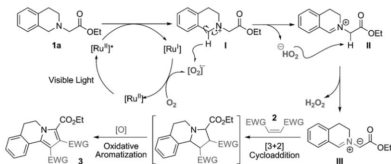
Scheme 1. Photocatalytic oxidation/cycloaddition/aromatization sequence. EWG = electron-withdrawing group.
