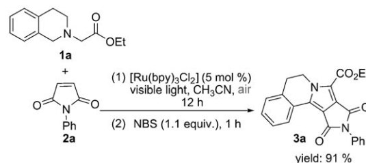
Scheme 2. Reaction system open to air.
