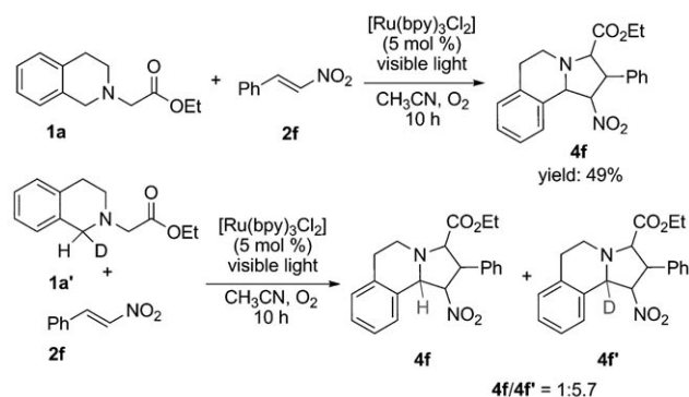
Scheme 3. Mechanistic studies.
